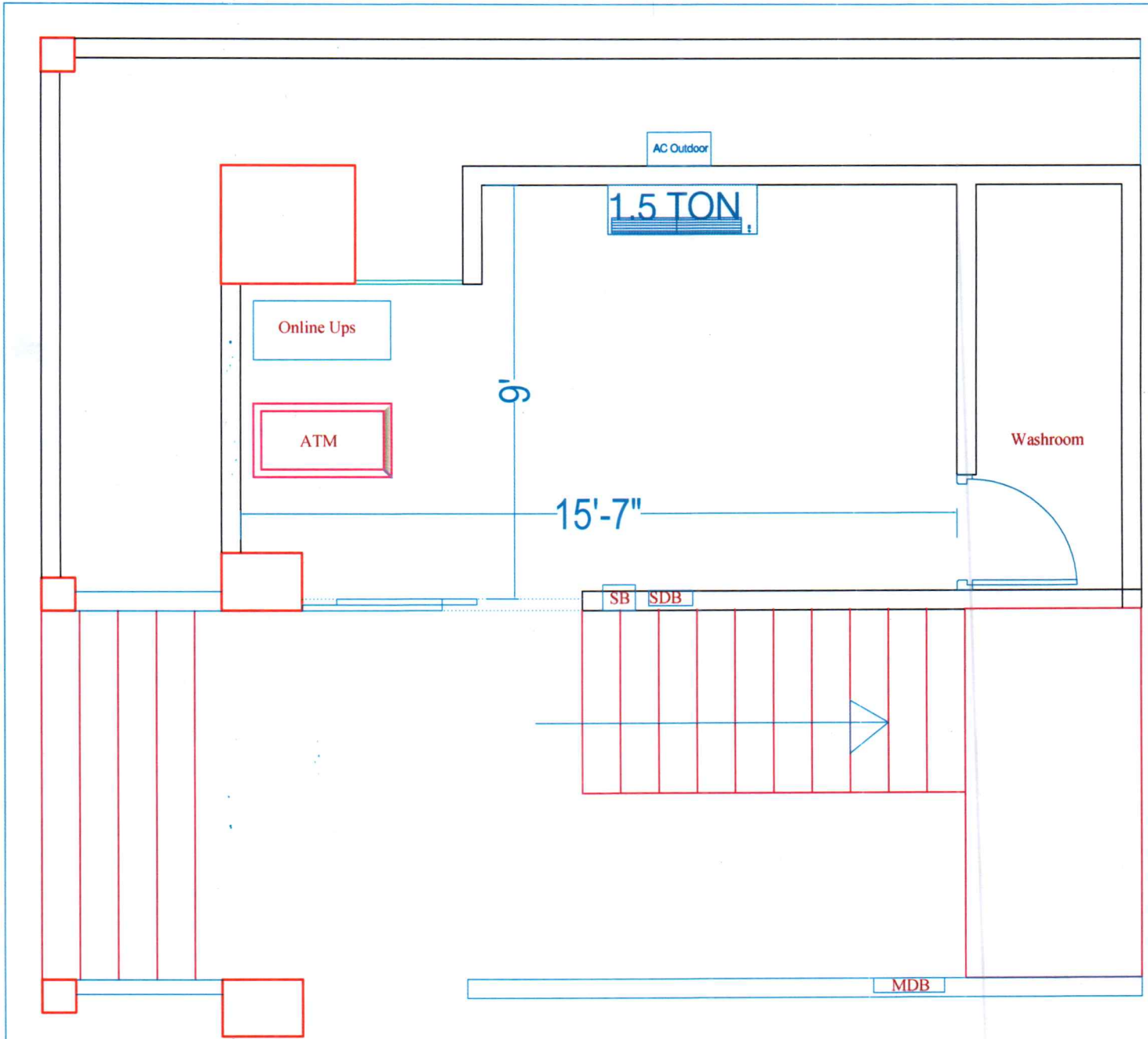
Proposed ATM Booth-POHS 1,Purbachal
